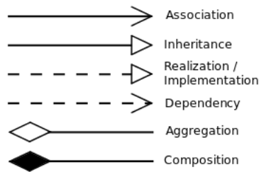
Figure 9.2: UML logical connectors
