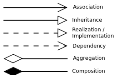
Figure 2.1: UML logical connectors
