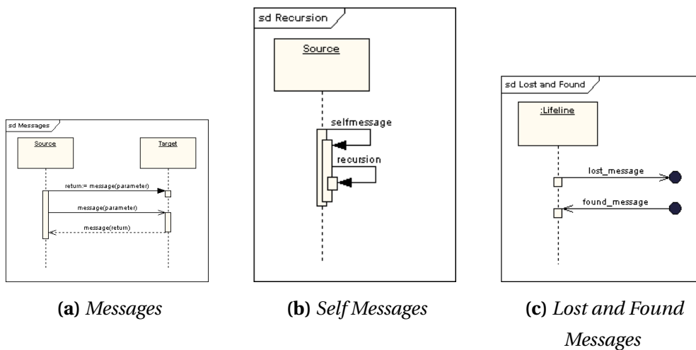
Figure 2.4: Sequence Diagram Messages
