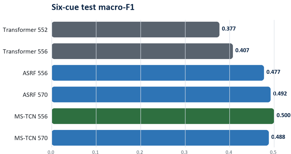
Figure 2. Temporal architecture contributes substantially more than adding expression and handcrafted dynamics.
