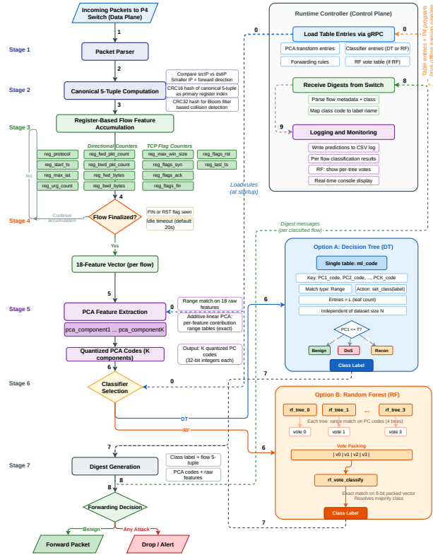
Fig. 2. In-network inference pipeline. Each finalized flow is canonicalized, accumulated into 18 bidirectional flow features, projected through the additive PCA range tables into K quantized PCA codes, classified by a Decision Tree or 4-tree Random Forest, and emitted as a digest to the controller.
