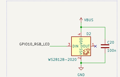
RGB LED
