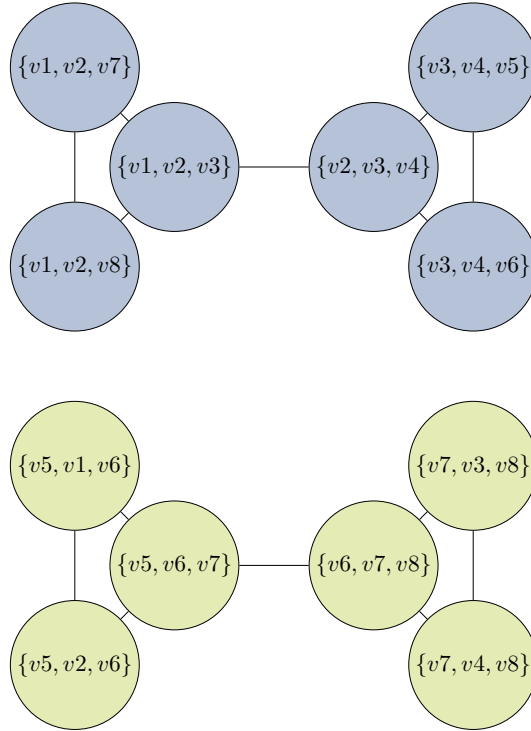
Figure 11: The line graph \Lambda_2(G) of the graph G in Figure 10. The vertices are coloured according to the colour of the corresponding edge in Figure 10.
