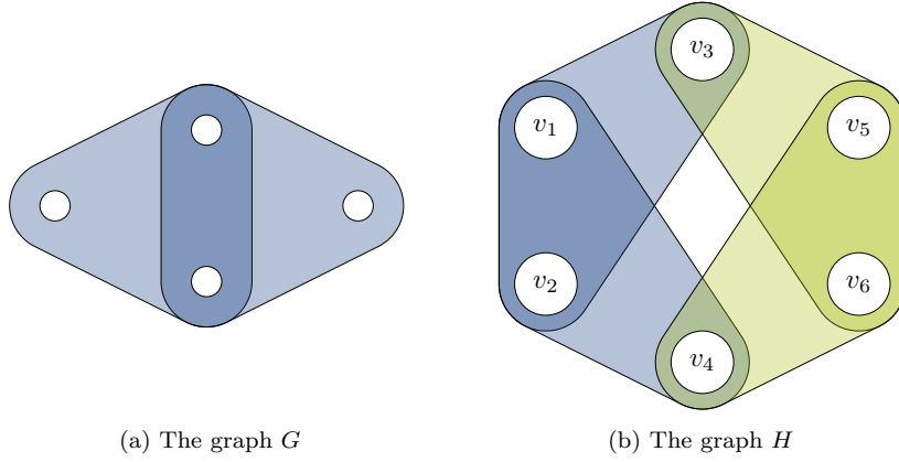
Figure 3: Consider the situation where \mathfrak{R} consists of just E_3 , the graph on three vertices with one edge containing all three vertices, and G and H are as in the figures. As we have seen previously, we will have \Phi_{\mathfrak{R}}(G) isomorphic to G and likewise for H . It is clear that \Phi_{\mathfrak{R}}(G) is 2-ly connected. \Lambda_2(\Phi_{\mathfrak{R}}(H)) has two connected components, one containing the blue edges and one containing the green edges, and so \Pi_{\mathfrak{R},2}(H) will have two parts, \{v_1, v_2, v_3, v_4\} and \{v_3, v_4, v_5, v_6\} . However, when we add G into \mathfrak{R} , this will add some new edges into \Phi_{\mathfrak{R} \cup \{G\}}(H) , with vertex sets v_1, v_2, v_3, v_4 and v_3, v_4, v_5, v_6 . (There will be 4 edges with each vertex set, due to the symmetries of G .) These two edge sets overlap in v_3 and v_4 , and so these edges form a connected component of \Lambda_2(\Phi_{\mathfrak{R} \cup \{G\}}(H)) , which will be sent to a part containing all vertices. Thus \Pi_{\mathfrak{R} \cup \{G\},2}(H) is not equal to \Pi_{\mathfrak{R},2}(H) .
