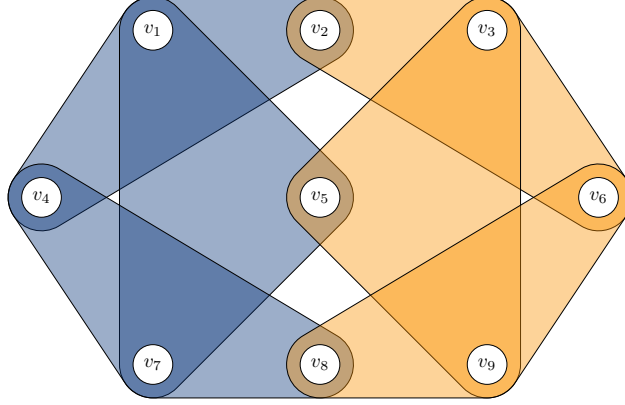
Figure 7: The graph G used in the proof of Lemma B.1.
