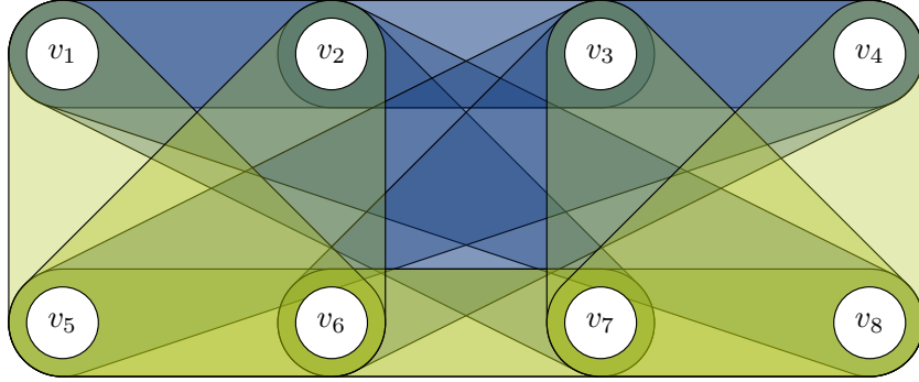
Figure 10: The graph G used in the proof of Example C.1.
