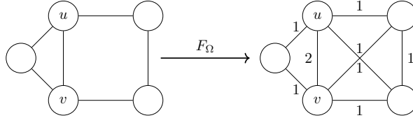
Figure 3: An example of a graph showing that \Omega = \{(K_3, 1), (C_4, 1)\} does not give an excisive clustering functor at threshold 1.5.
