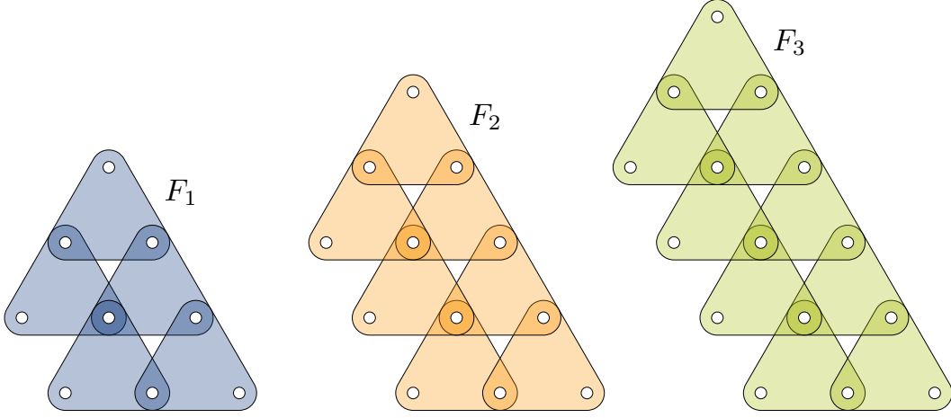
Figure 9: The graph family F_i used in the proof of Lemma B.1, illustrated by its first three members.
