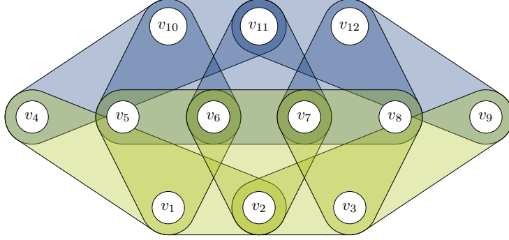
Figure 10: The graph G_1 used in the proof of Lemma B.1. This graph contains two copies of F_1 , corresponding to the green and the blue edges. Here, the vertices v_4 and v_9 are the leftmost column in the standard drawing of F_1 (Figure 9), and the vertices v_5, v_6, v_7 and v_8 are the rightmost column. The vertices v_1, v_2, v_3 are the middle column in the green copy of F_1 , and the vertices v_{10}, v_{11}, v_{12} are the middle column in the blue copy of F_1 .
