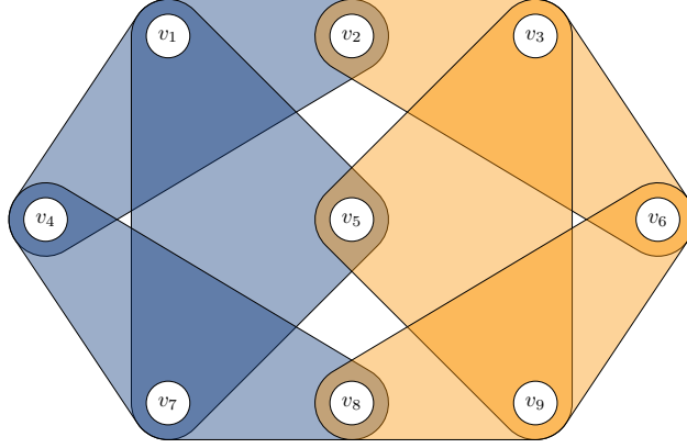
Figure 8: The graph G used in the proof of Lemma B.1.
