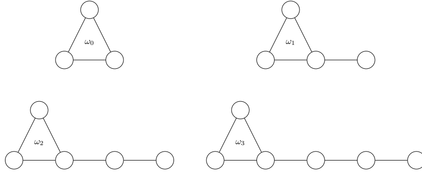
Fig. 2: The family of graphs \{\omega_i\}_{i=0}^3 .
