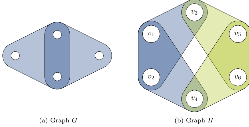
Figure 2: Consider the situation where \mathfrak{R} consists of just one graph on three vertices with one edge containing all three vertices, and G and H are as in the figures. It is clear that \Phi_{\mathfrak{R}}(G) is k -ly connected. \Lambda_2(\Phi_{\mathfrak{R}}(H)) has two connected components, one containing the blue edges and one containing the green edges, and so \Pi_{\mathfrak{R},2}(H) will have two parts, \{v_1, v_2, v_3, v_4\} and \{v_3, v_4, v_5, v_6\} .
