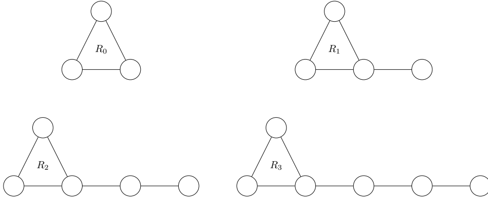
Figure 3: The family of graphs \{R_i\}_{i=0}^3 .
