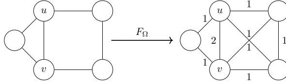
Figure 6: An example of a graph showing that \mathfrak{R} = \{(K_3, 1), (C_4, 1)\} does not give an excisive clustering functor at threshold 1.5.
