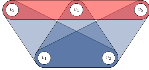
Figure 5: An example of a graph G with a connected component p (here, the entire vertex set) where p'' is a strict subset of p' , in the notation of the proof of Lemma 5.5. In particular, we note that p'' consists of the three blue edges, which form a clique in the line graph since they all overlap in the vertices v_1 and v_2 , but the line graph also has an isolated vertex corresponding to the red edge. This red edge is in p' , but not in p'' , and will be sent to a strict subpart of p by \Upsilon .
