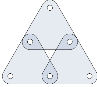
Figure 7: The graph D used in the proof of Lemma 5.16.
