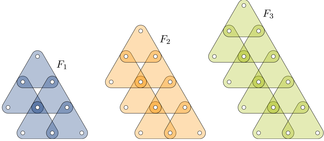
Figure 8: The graph family F_i used in the proof of Lemma B.1, illustrated by its first three members.
