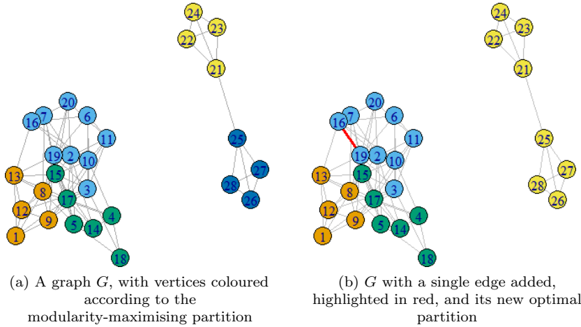
Figure 1: An illustration of the resolution limit issue with modularity.
