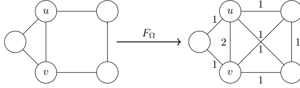
Figure 4: An example of a graph showing that \mathfrak{R} = \{(K_3, 1), (C_4, 1)\} does not give an excisive clustering functor at threshold 1.5.
