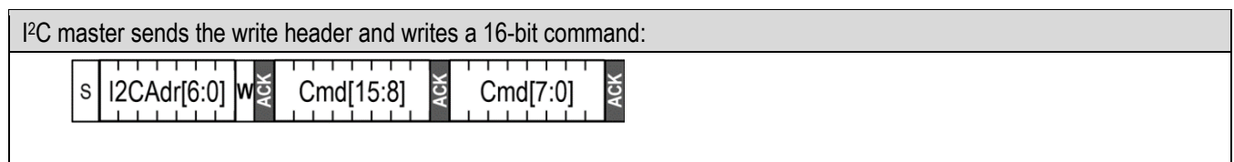
Figure 2: I 2 C sequences to send a command without an argument to the sensor.
