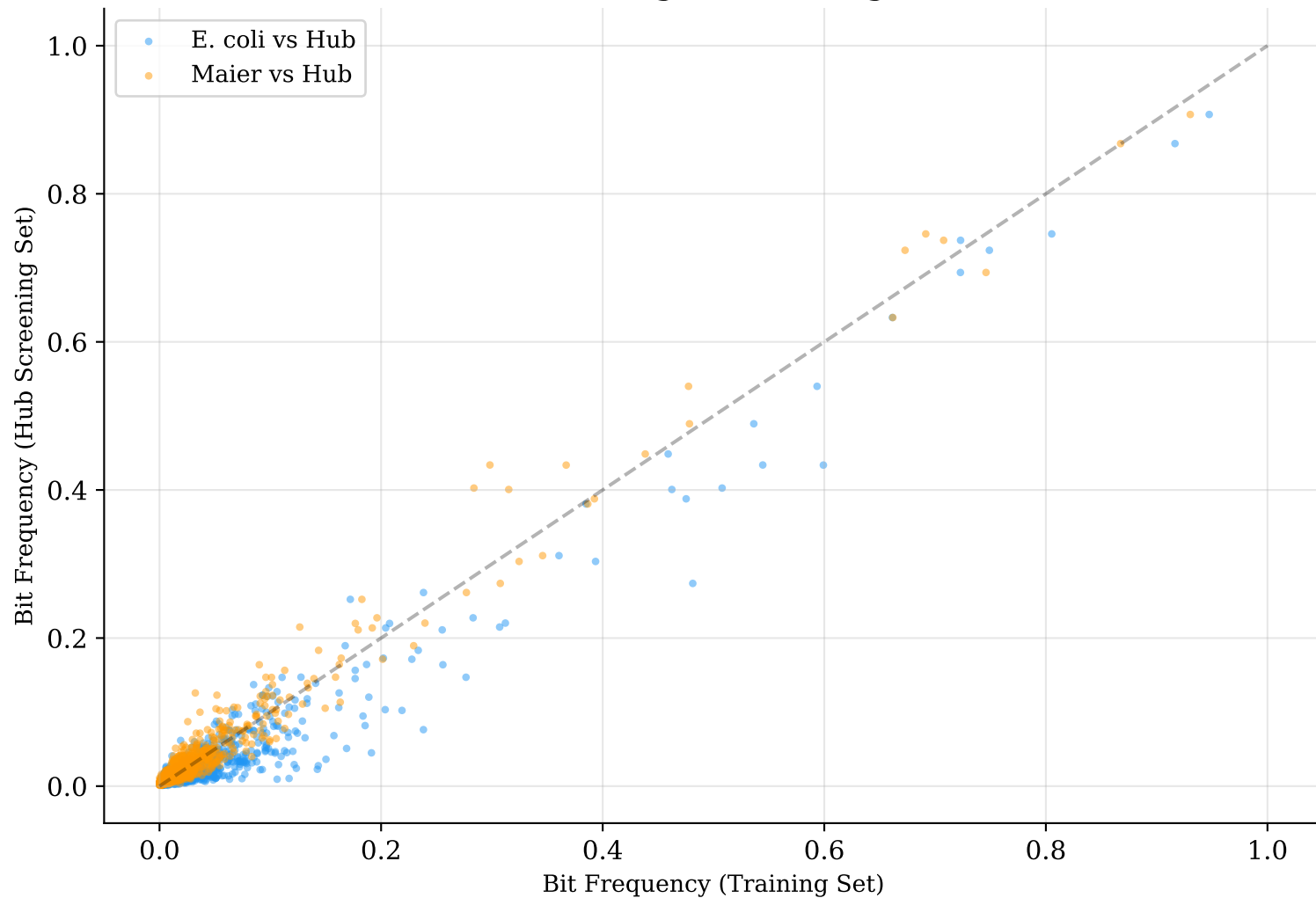
Fingerprint Bit Frequency: Training vs Screening
