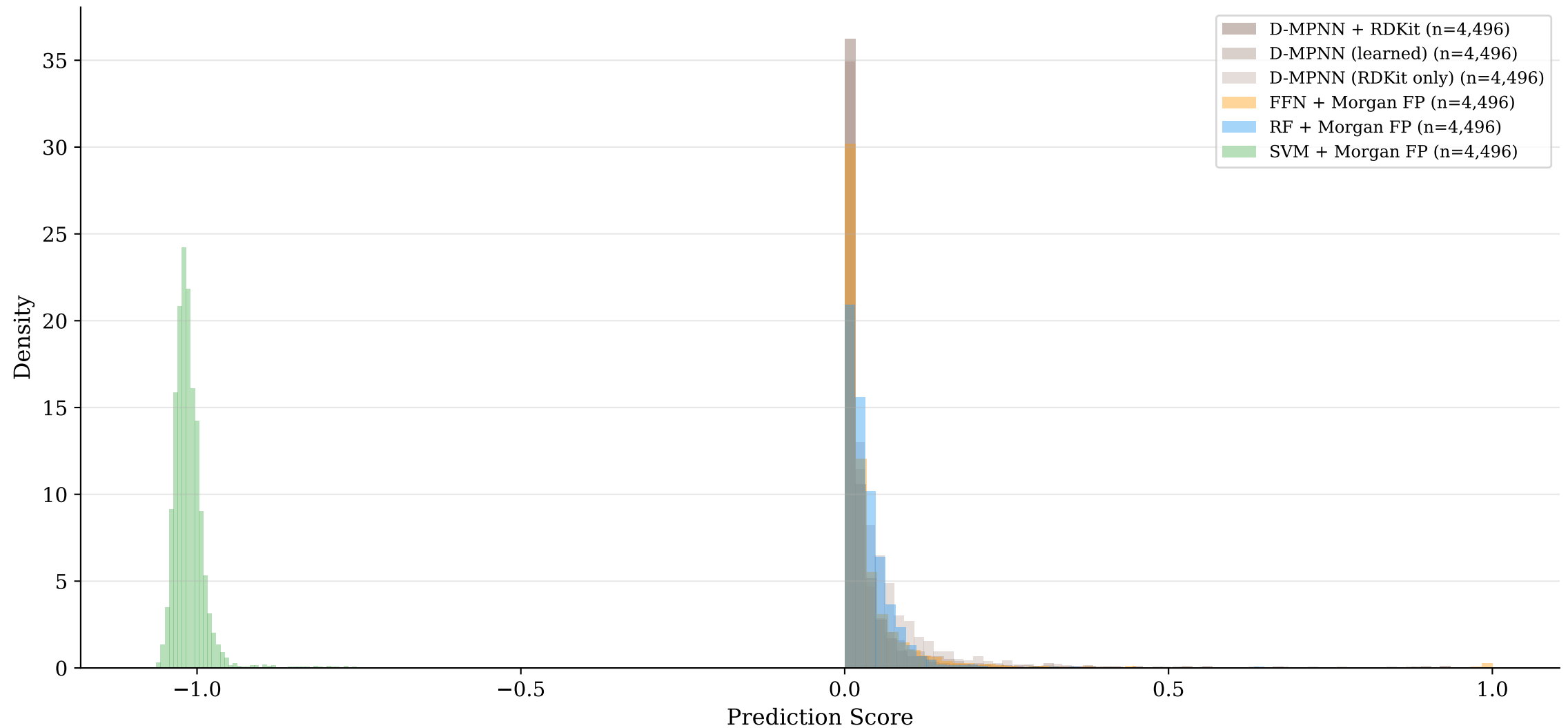
Stokes et al.: Prediction Score Distributions Across Model Architectures
