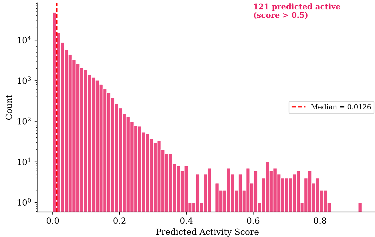
Wong Broad800 Predictions (n=99,998)
