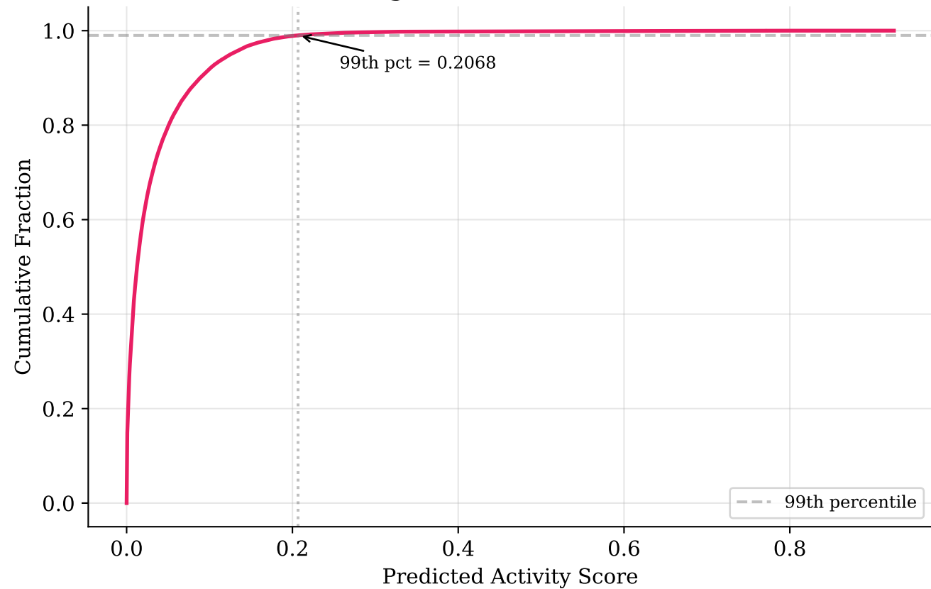
Wong Broad800: Score CDF
