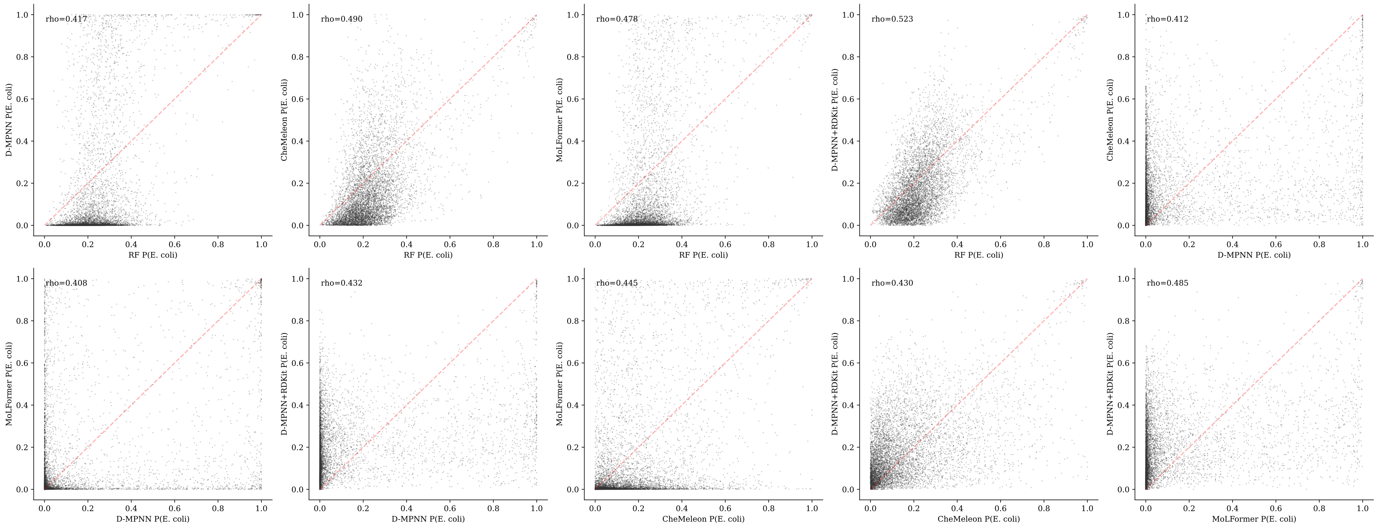
Pairwise Raw P(E. coli) Agreement
