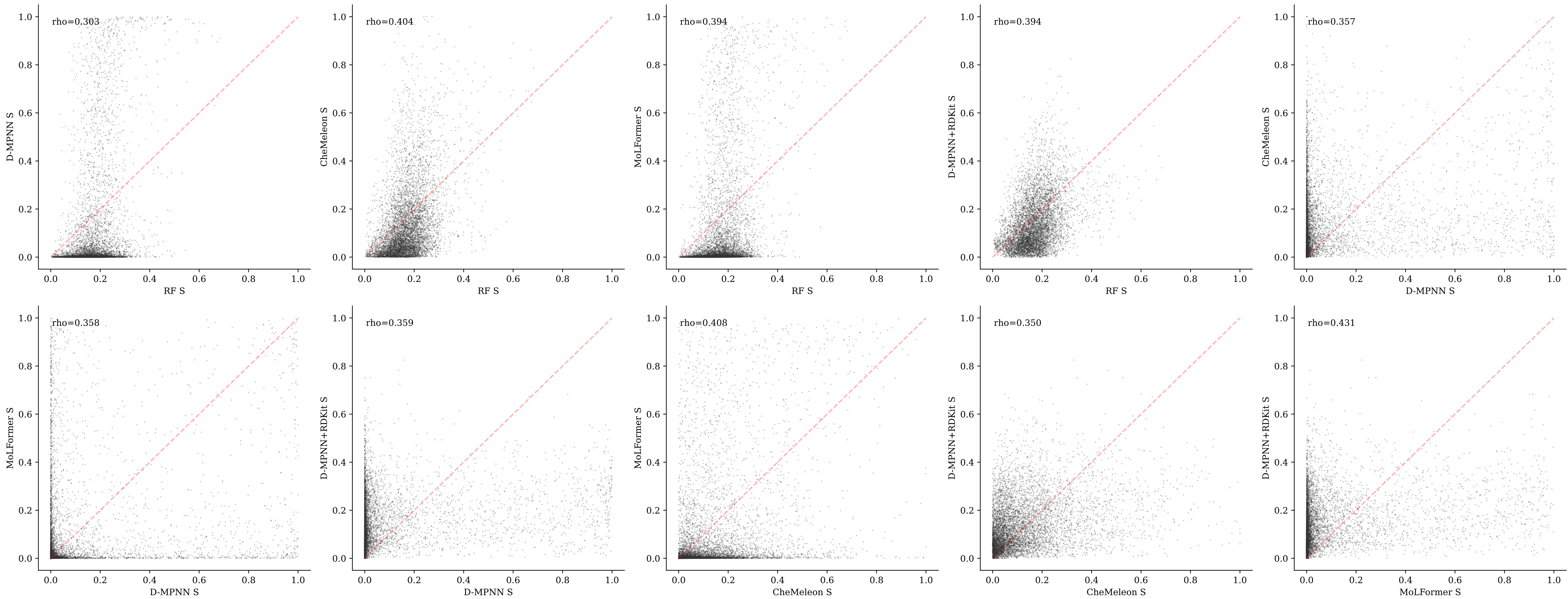
Pairwise Selectivity Score Agreement (E. coli, t=10)
