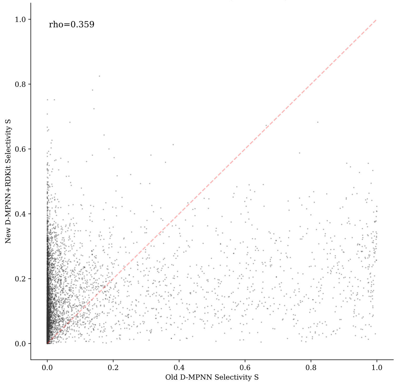
Old vs New D-MPNN (E. coli, t=10)
