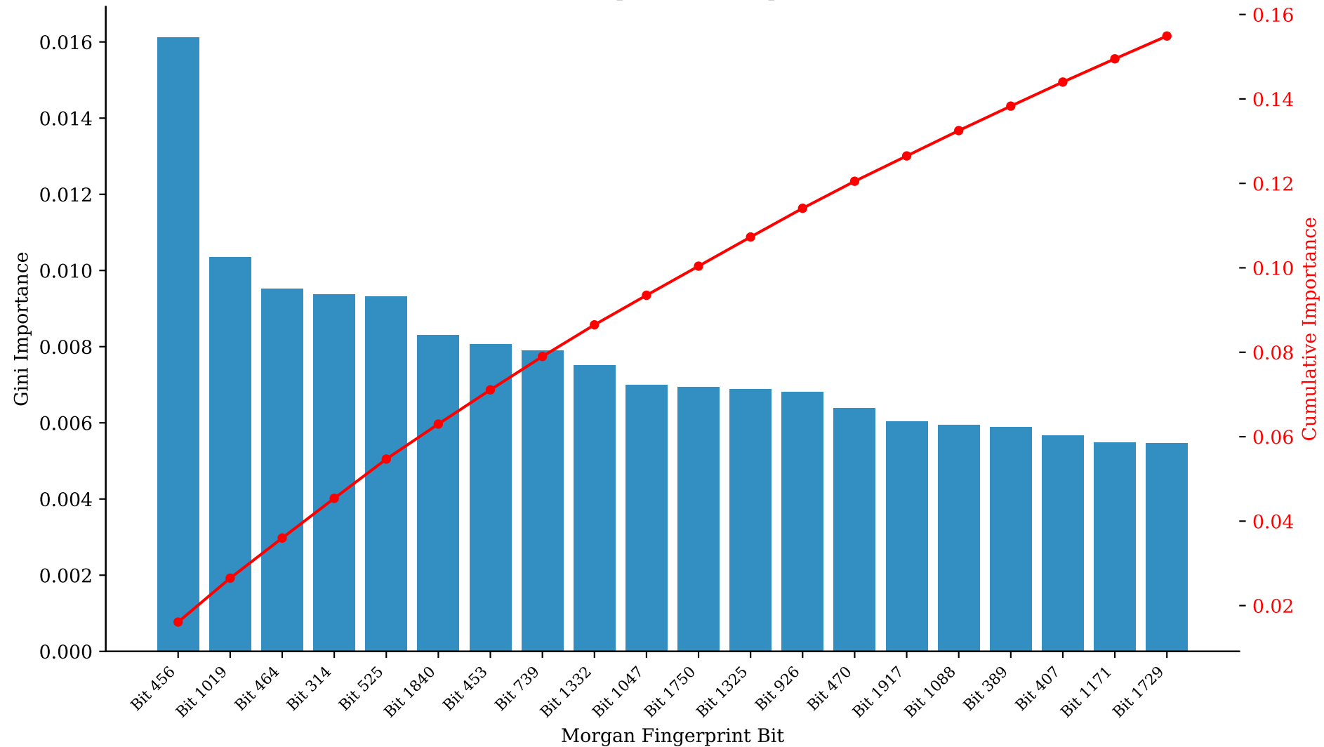
RF E. coli Model: Top 20 Most Important Features
