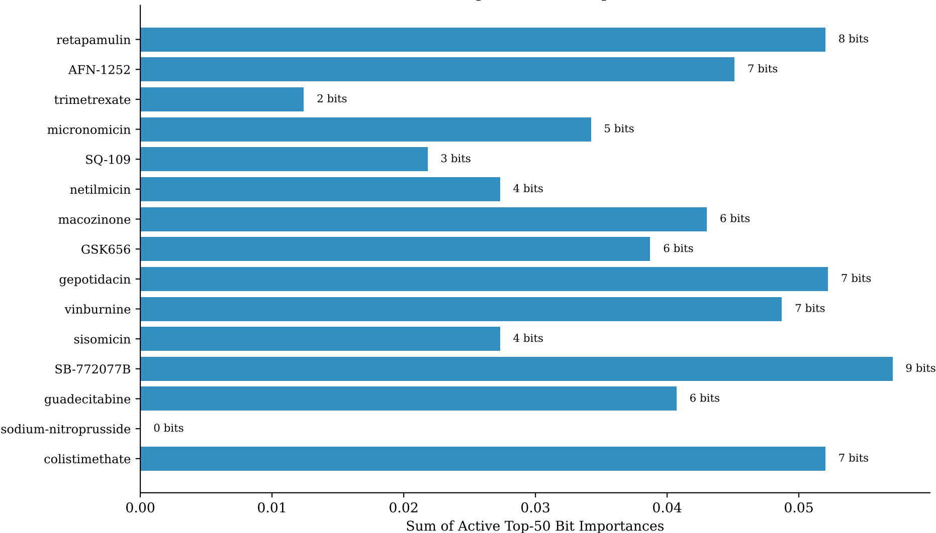
RF: Feature Importance Mass per Candidate
