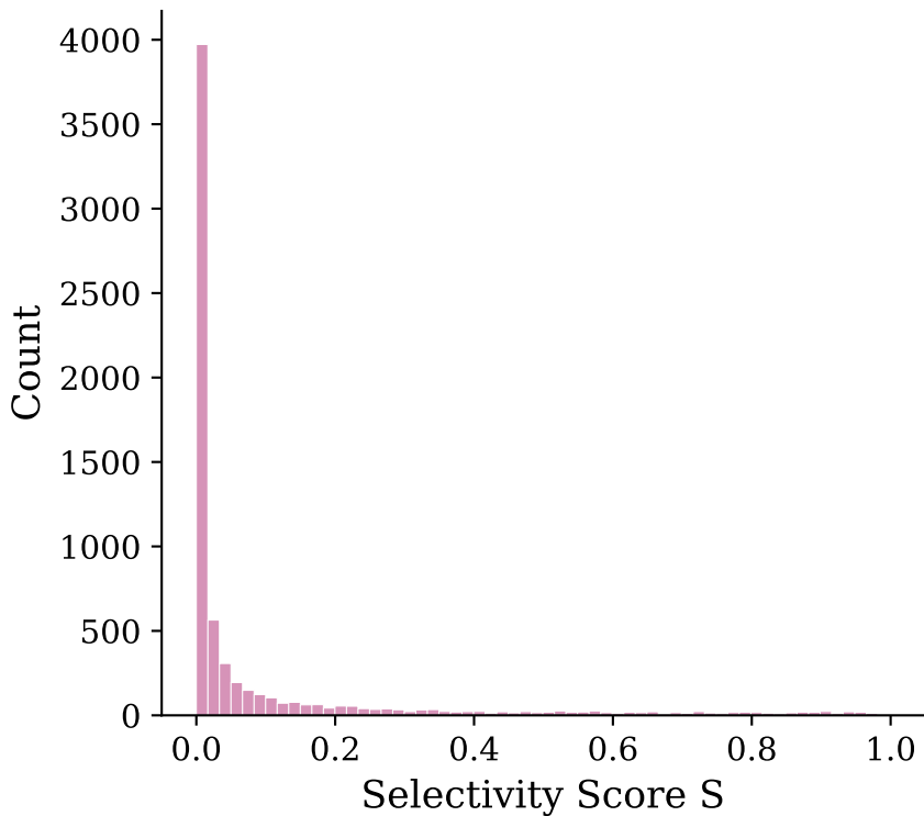
A. S distribution (MolFormer, E. coli, t=10)
