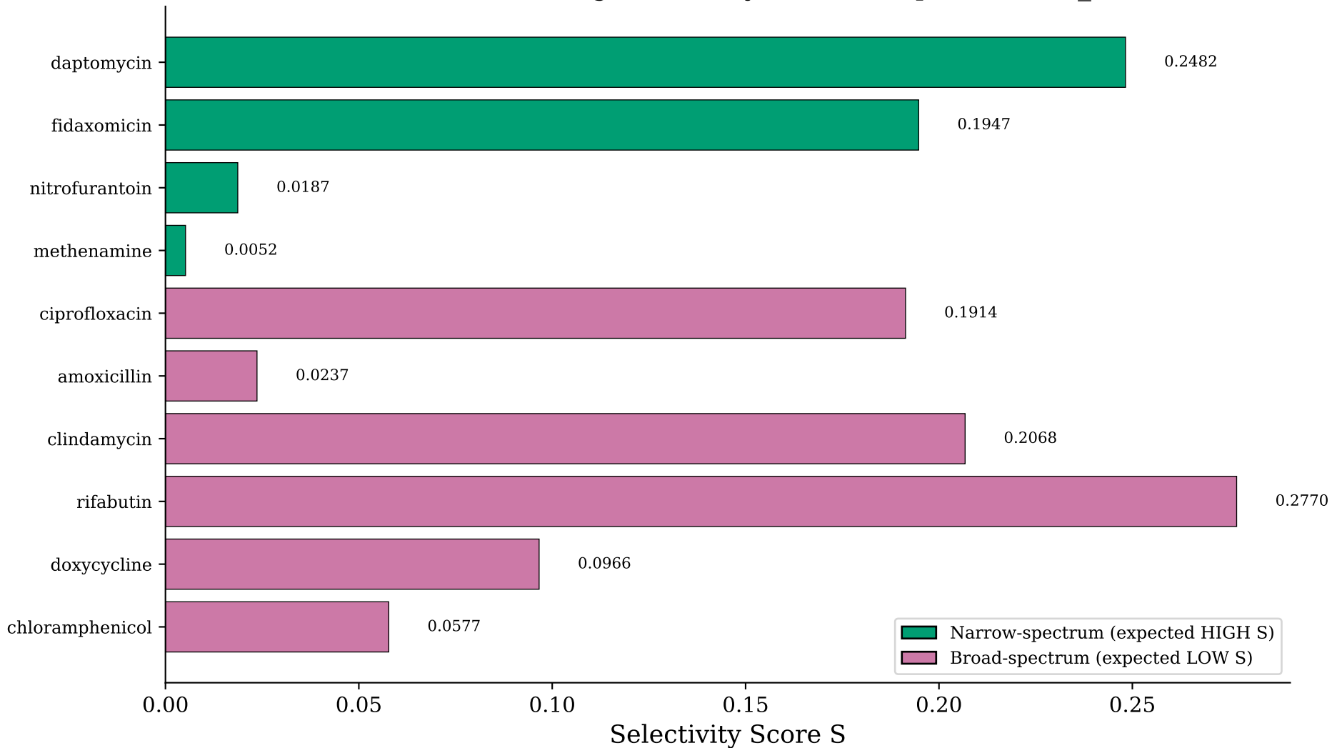
CheMeleon: Validation Drug Selectivity (mtb, t=5, p=0.7619, r_rb=0.250)
