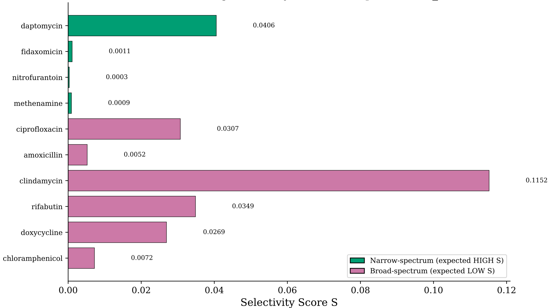
D-MPNN: Validation Drug Selectivity (ecoli, t=10, p=0.9429, r_rb=0.583)
