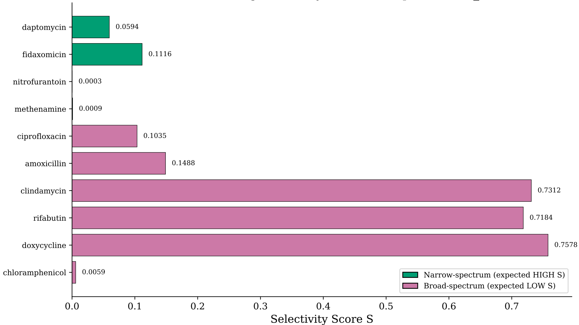
D-MPNN: Validation Drug Selectivity (ecoli, t=20, p=0.9810, r_rb=0.750)
