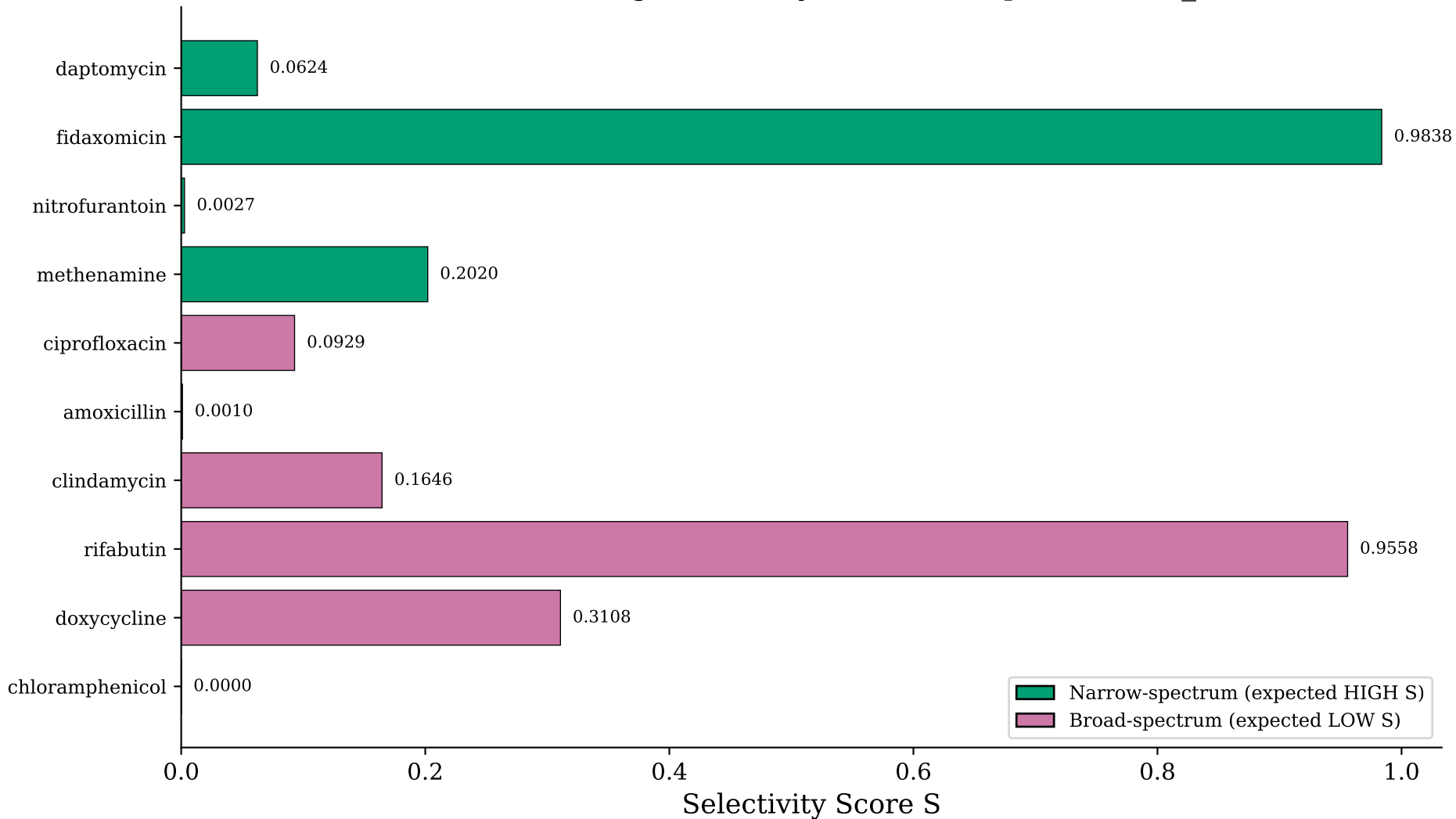
D-MPNN: Validation Drug Selectivity (mtb, t=20, p=0.3810, r_rb=-0.167)
