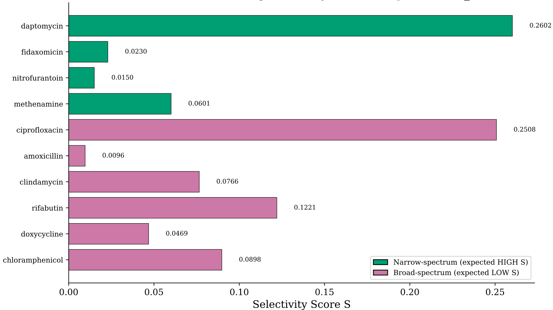
D-MPNN+RDKit: Validation Drug Selectivity (ecoli, t=5, p=0.6952, r_rb=0.167)
