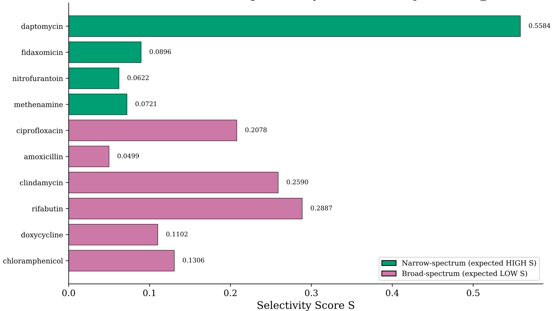
D-MPNN+RDKit: Validation Drug Selectivity (saureus, t=10, p=0.7619, r_rb=0.250)
