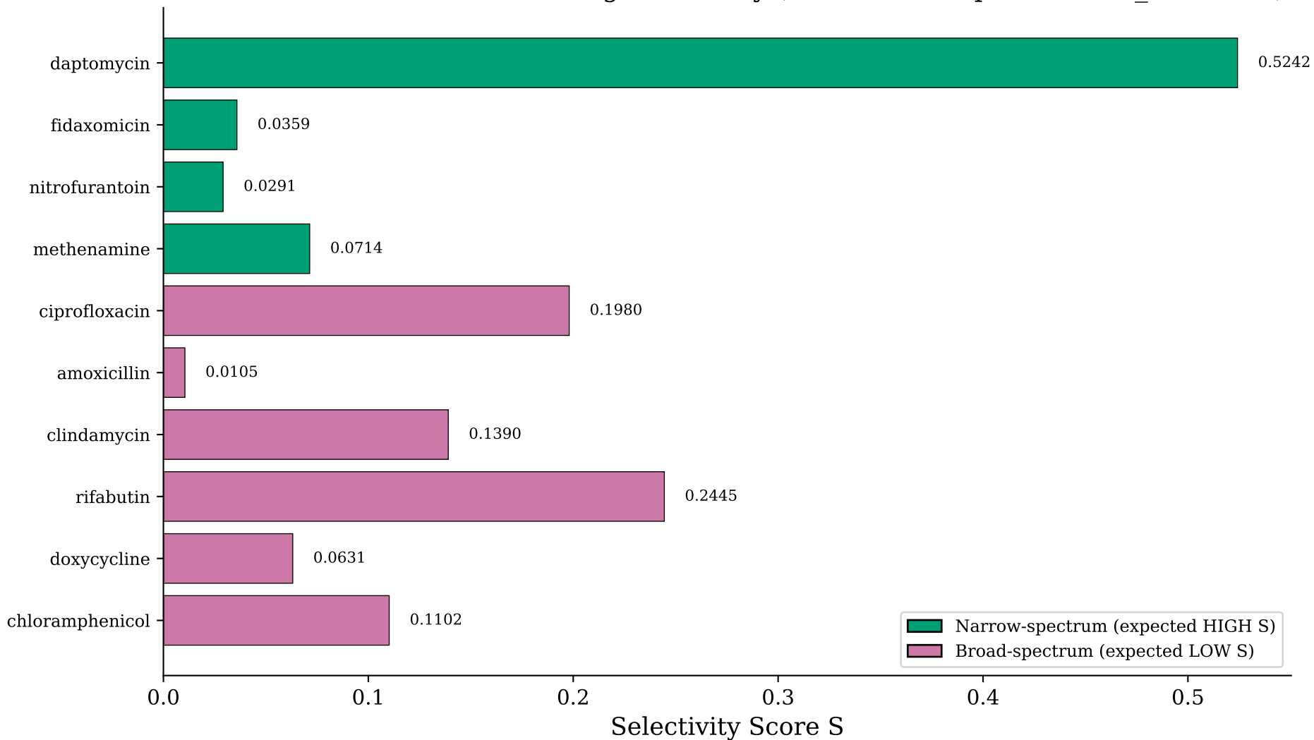
D-MPNN+RDKit: Validation Drug Selectivity (saureus, t=5, p=0.6952, r_rb=0.167)
