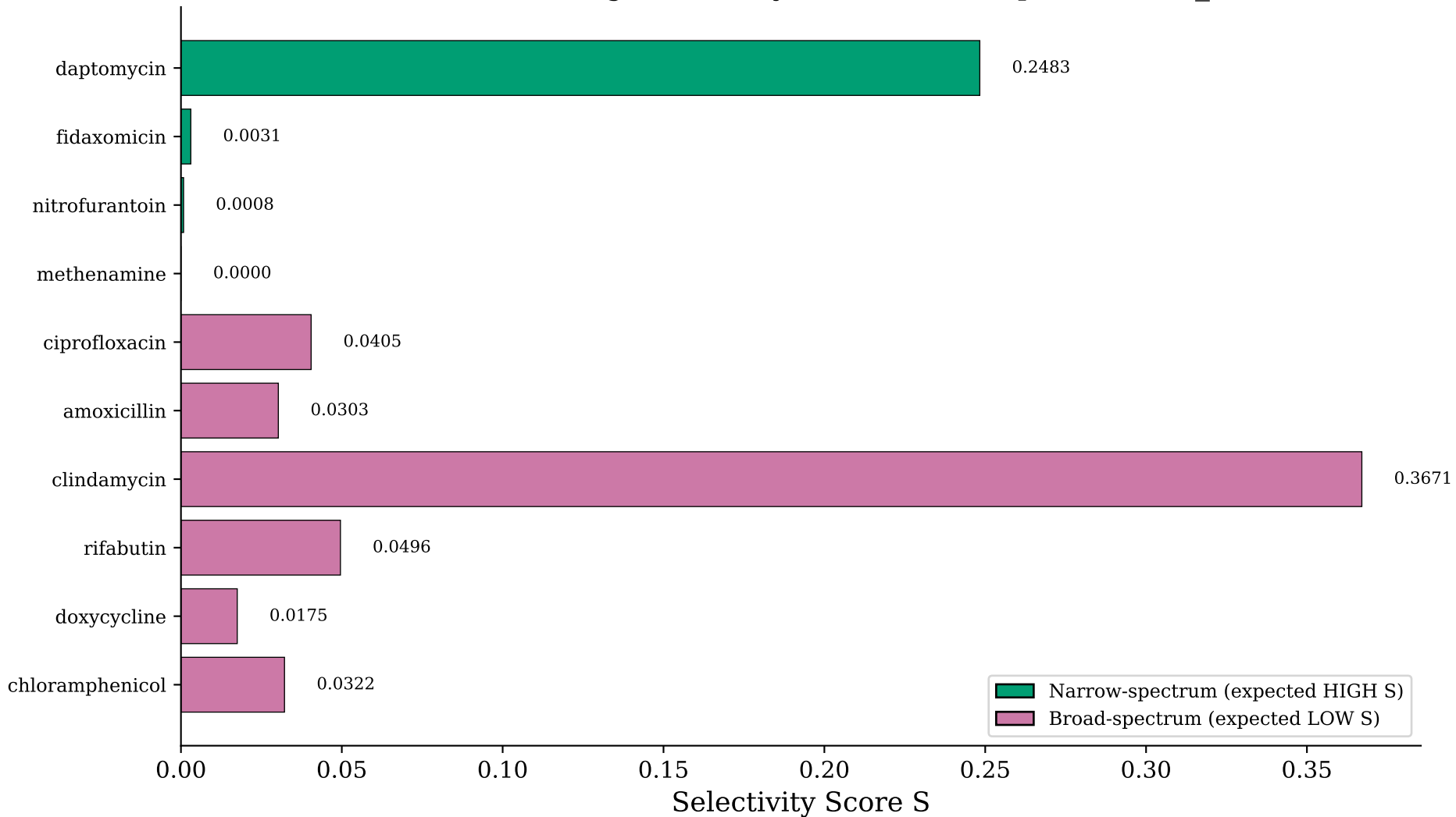
D-MPNN: Validation Drug Selectivity (saureus, t=5, p=0.9429, r_rb=0.583)
