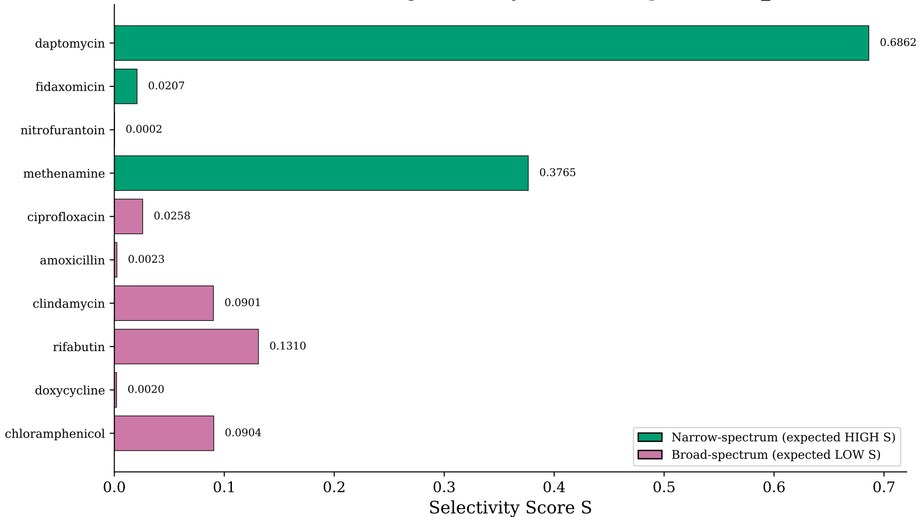
MoLFormer: Validation Drug Selectivity (ecoli, t=10, p=0.3810, r_rb=-0.167)
