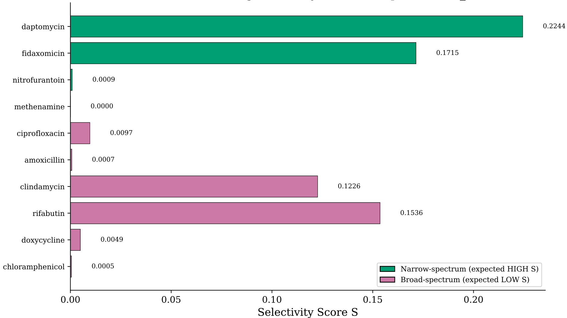
MolFormer: Validation Drug Selectivity (mtb, t=20, p=0.3810, r_rb=-0.167)
