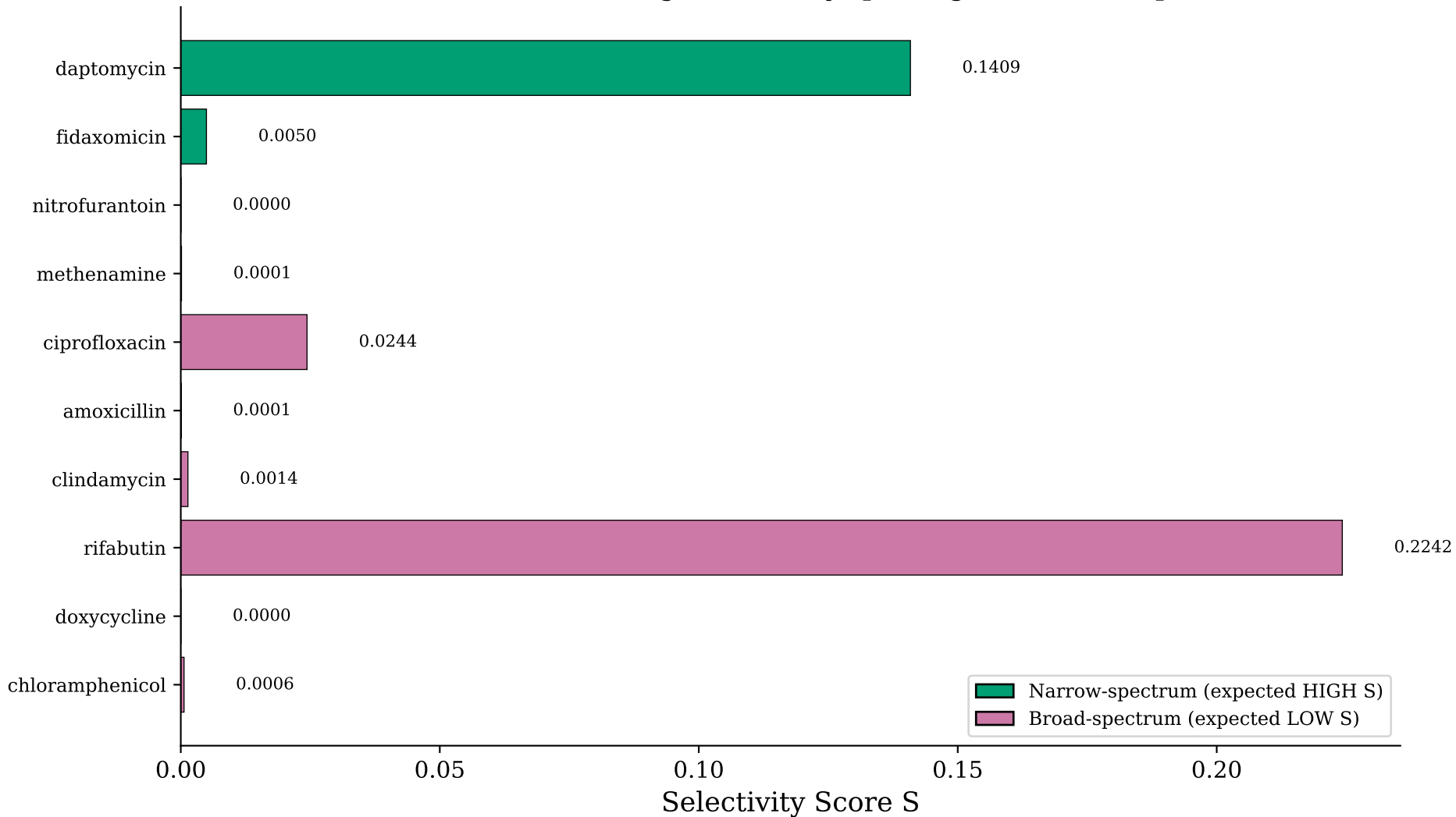
MoLFormer: Validation Drug Selectivity (paeruginosa, t=10, p=0.5429, )
