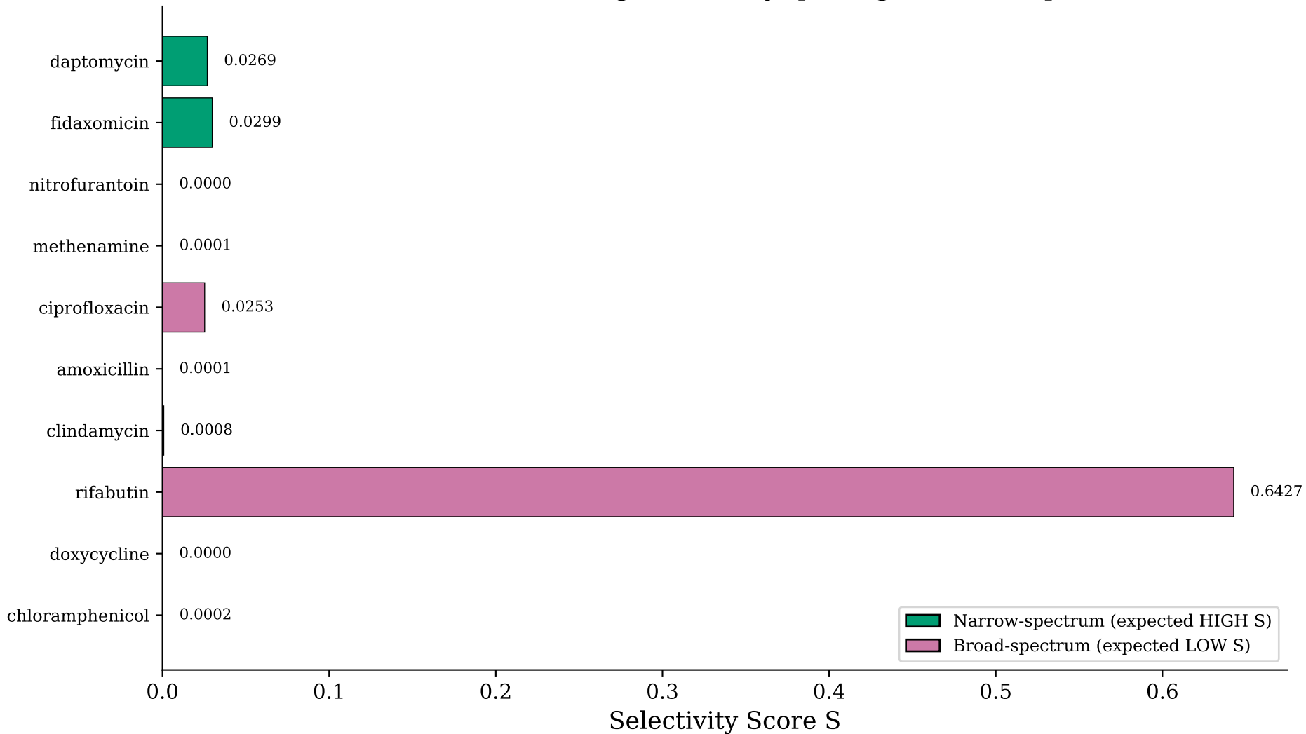
MoLFormer: Validation Drug Selectivity (paeruginosa, t=5, p=0.5429, )
