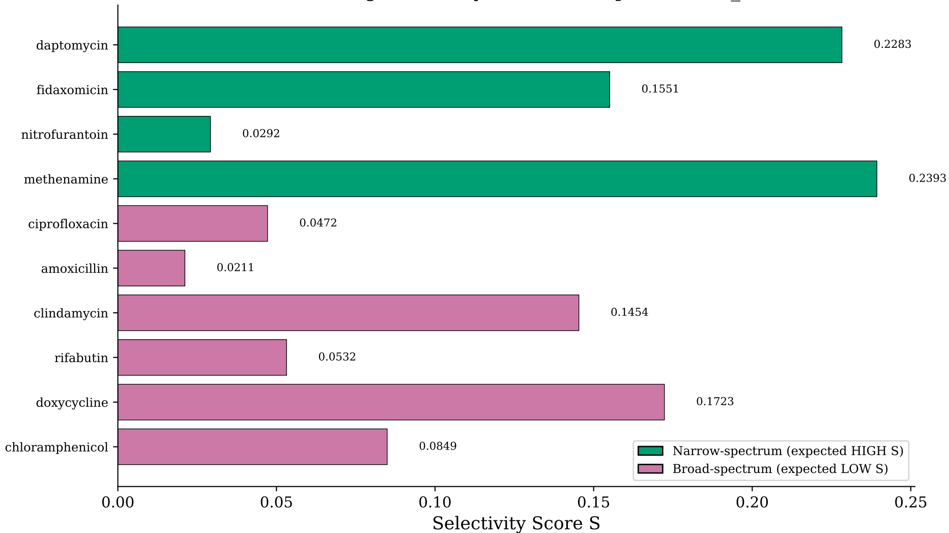
RF: Validation Drug Selectivity (ecoli, t=10, p=0.1286, r_rb=-0.500)
