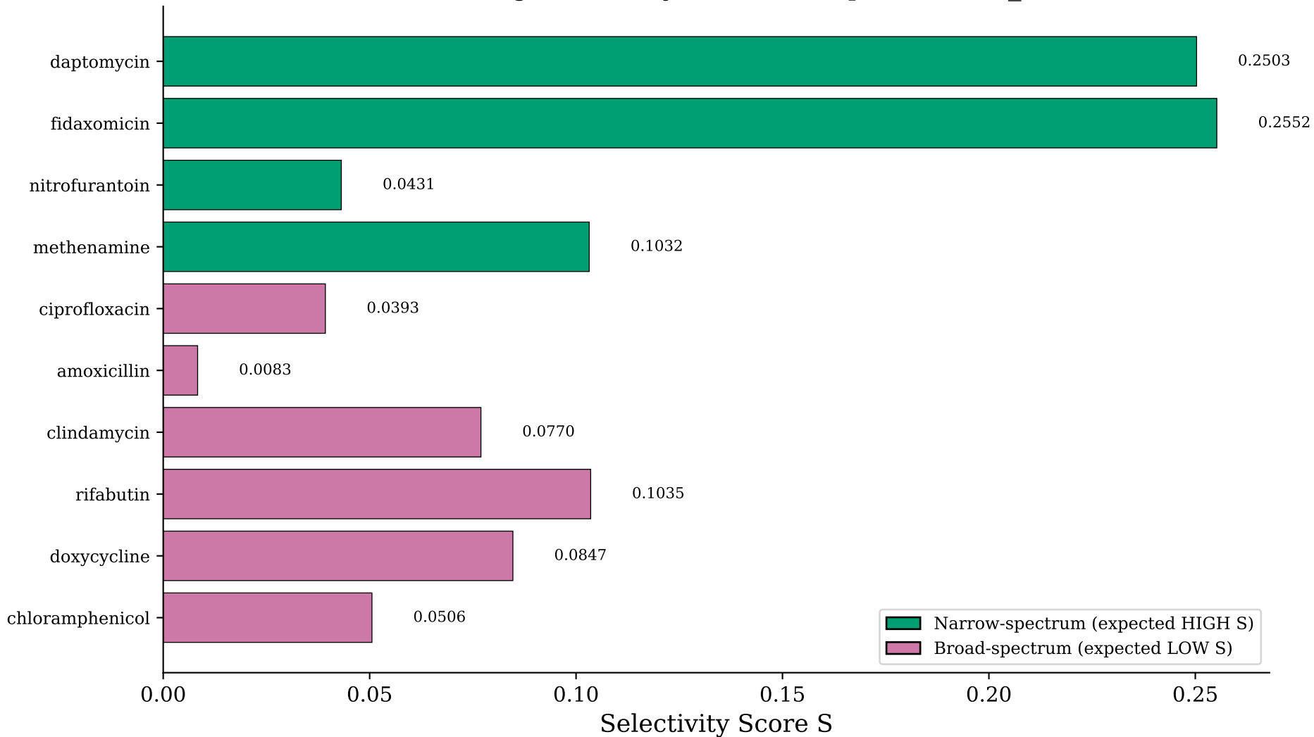
RF: Validation Drug Selectivity (mtb, t=10, p=0.0857, r_rb=-0.583)
