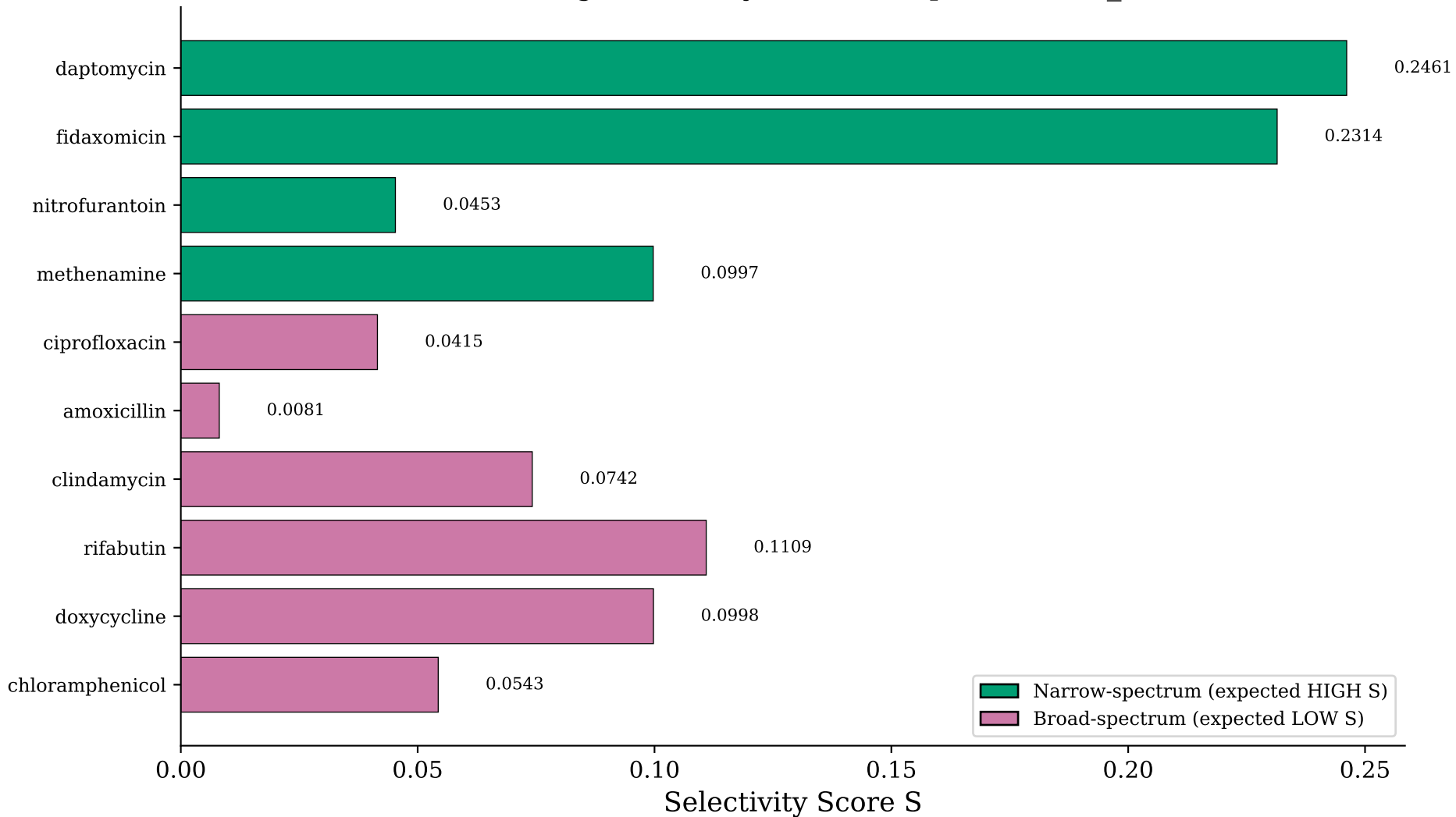
RF: Validation Drug Selectivity (mtb, t=5, p=0.1286, r_rb=-0.500)
