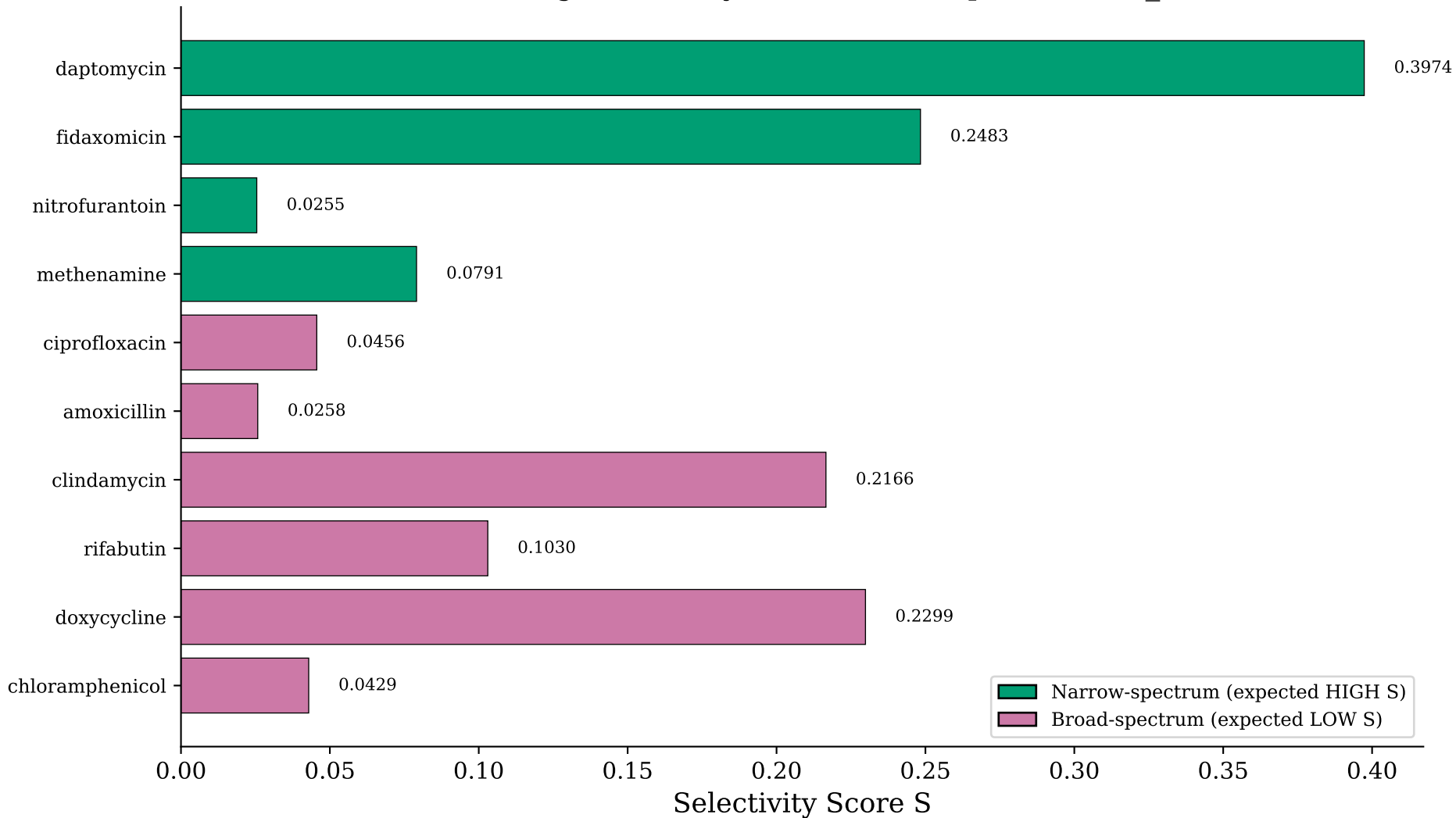
RF: Validation Drug Selectivity (saureus, t=5, p=0.3048, r_rb=-0.250)
