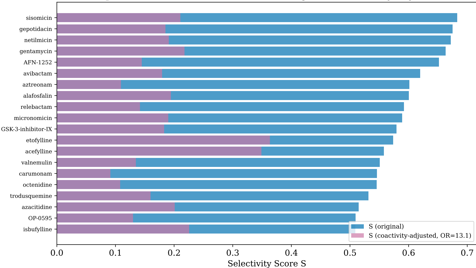
Top-20 RF Candidates (E. coli, t=10): Original vs Coactivity-Adjusted
