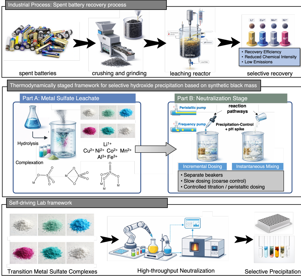
Figure 1: Process schematic for selective metal recovery from battery black mass. (Top) Industrial process: spent batteries mechanical preprocessing (crushing/grinding) leaching selective recovery. (Middle) Mechanistic framework: (A) multi-metal sulfate leachate chemistry (hydrolysis/complexation equilibria); (B) controlled neutralization strategies (incremental dosing vs instantaneous mixing) enabling thermodynamically staged hydroxide precipitation. (Bottom) Self-driving laboratory: Mixing transition metal sulfates with DI water robotic HTE neutralization inline ICP analytics selective precipitation screening.
