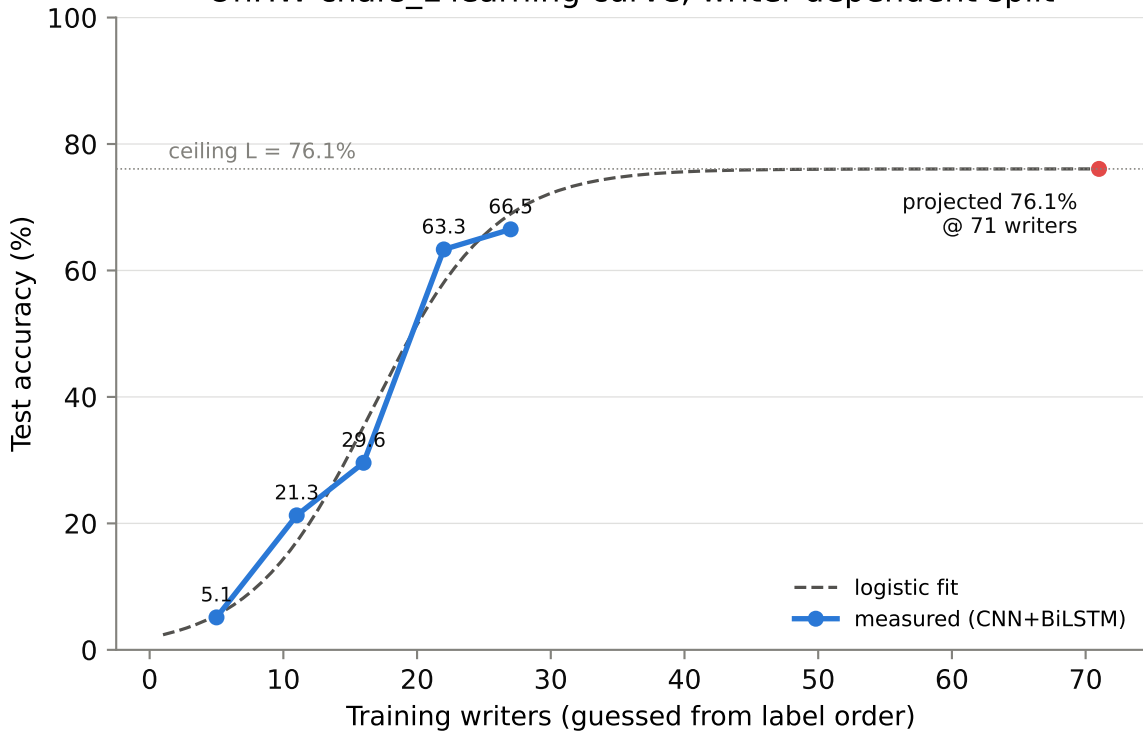
OnHW-chars_L learning curve, writer-dependent split
