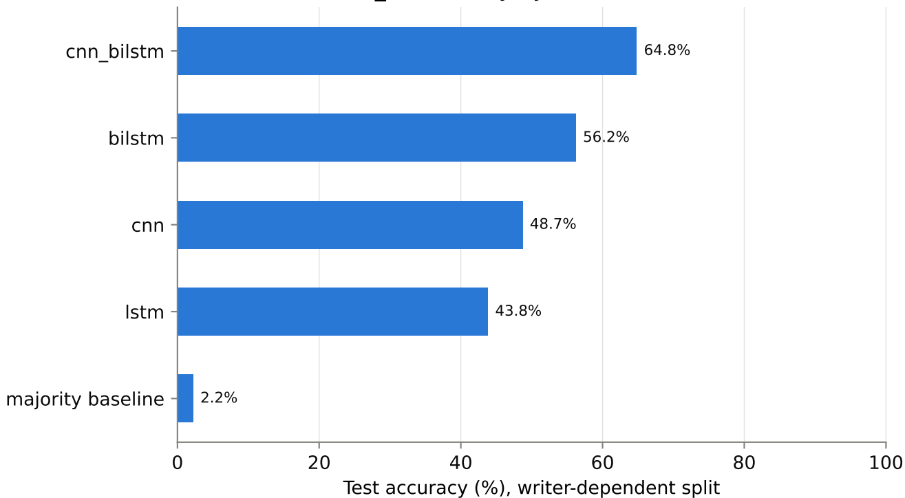
OnHW-chars_L: accuracy by architecture (52 classes)
