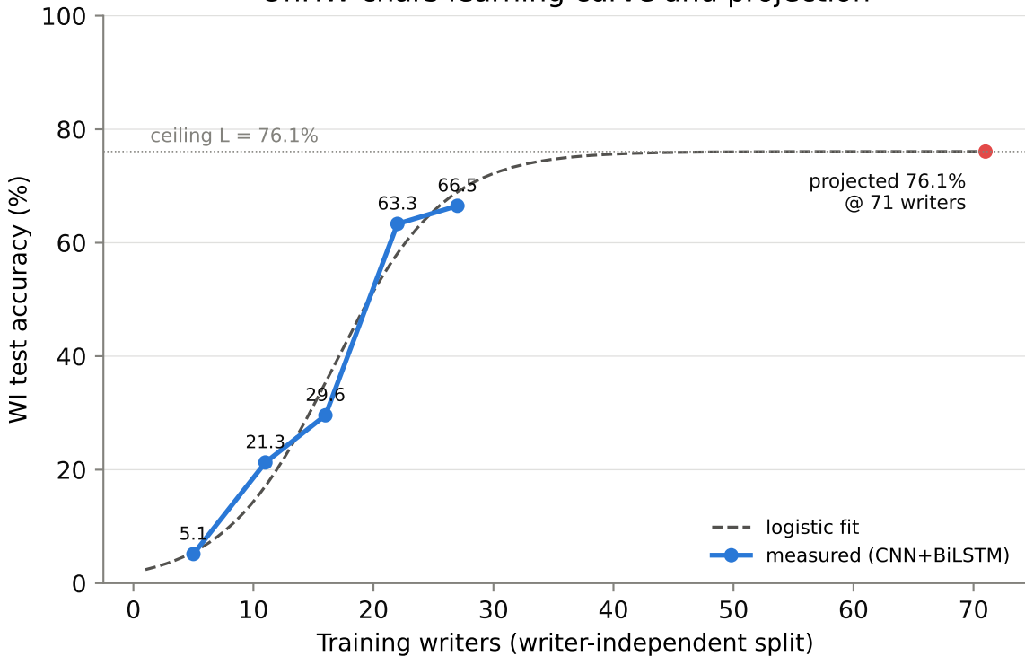
OnHW-chars learning curve and projection
