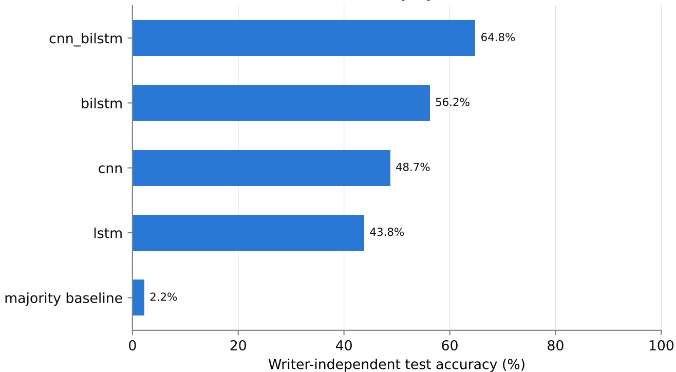
OnHW-chars: held-out accuracy by architecture (52 classes)
