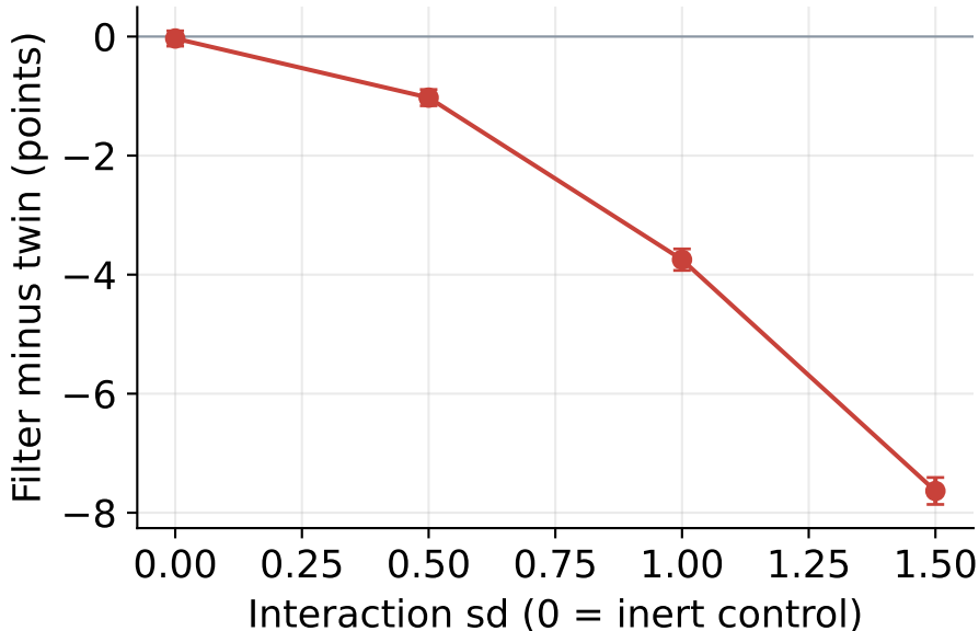
Penalty grows with interaction
