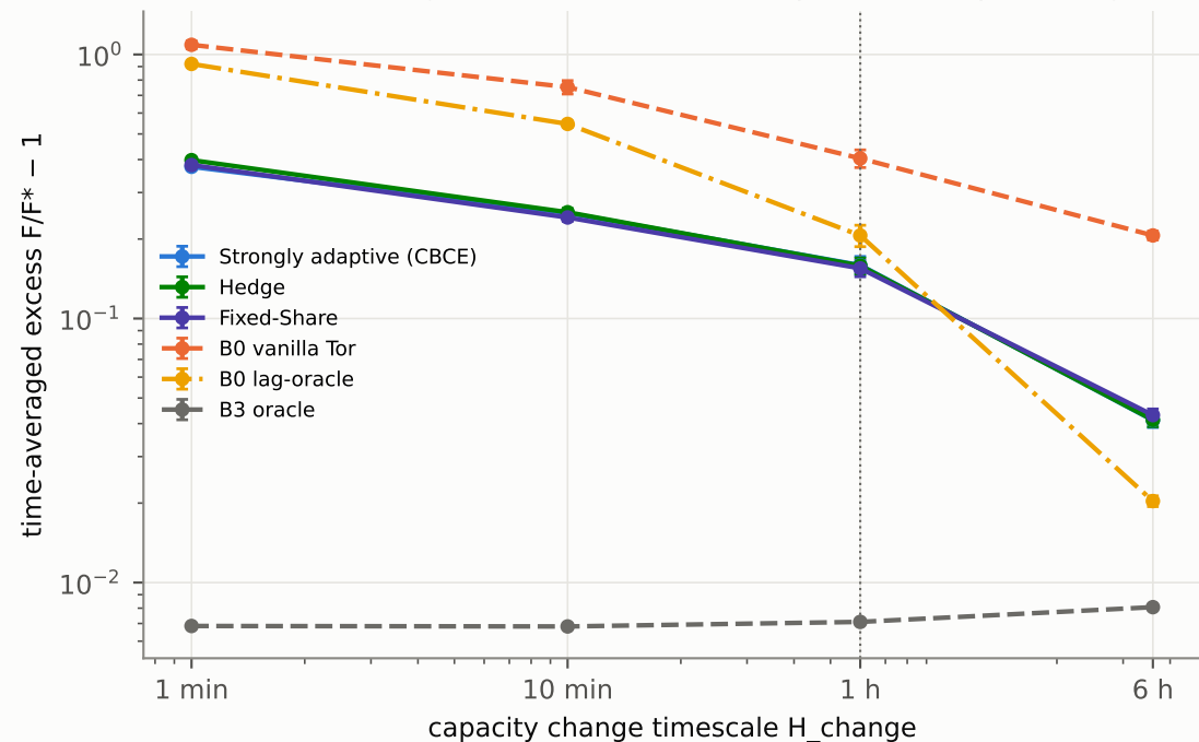
Excess vs. change timescale (30% of relays re-drawn per change)
