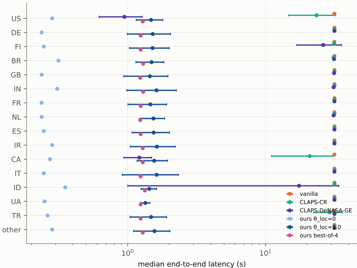
Median latency per client country (top 15 by Tor users)
