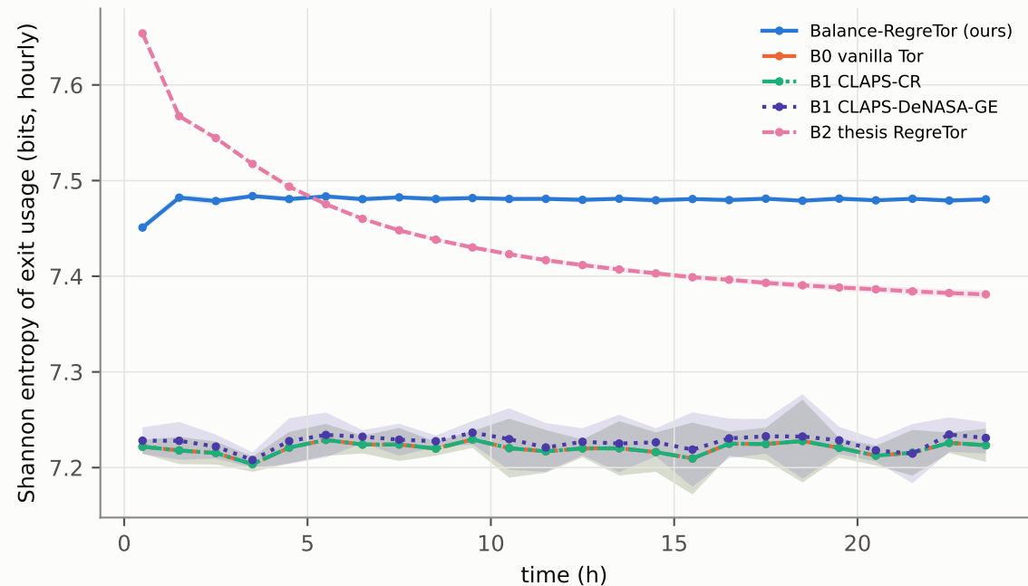
Exit-distribution entropy over time
